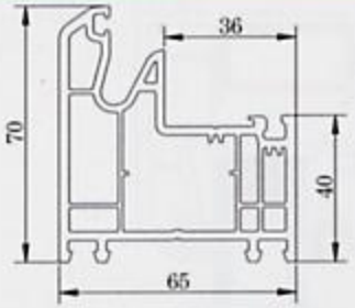
Outer Frame-BR65
