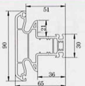
Frame Mullion-SE65
