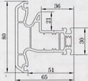
Frame Mullion-GT65
