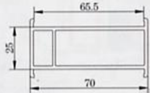
180° Corner-CE25
